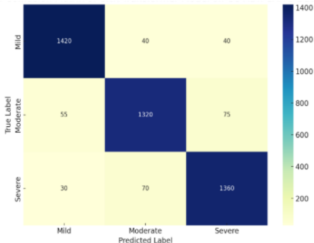
Fig.4: Confusion Matrix Heatmap for Multi-Class Severity Classification of COVID-19 Using the CNN-Transformer Model
