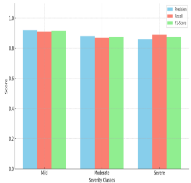
Fig.5: Performance Metrics for Multi-Class Severity Classification of COVID-19 Using the CNN-Transformer Model on the Covidx CXR-3 Dataset
