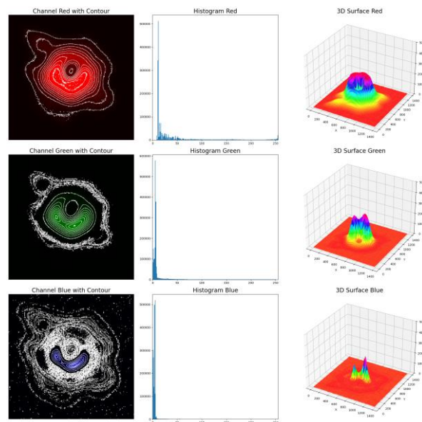
Fig. 2. Amplitude distribution in M87 EHT in RGB channels M87 EHT.
