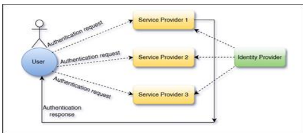
Fig. 2. Centralized Model (Source: Author)
